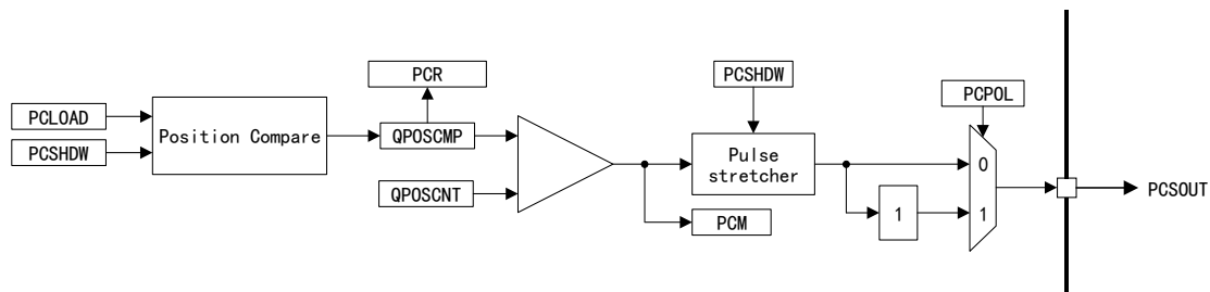
Figure 181 Structure Block Diagram of Position Compare Unit
