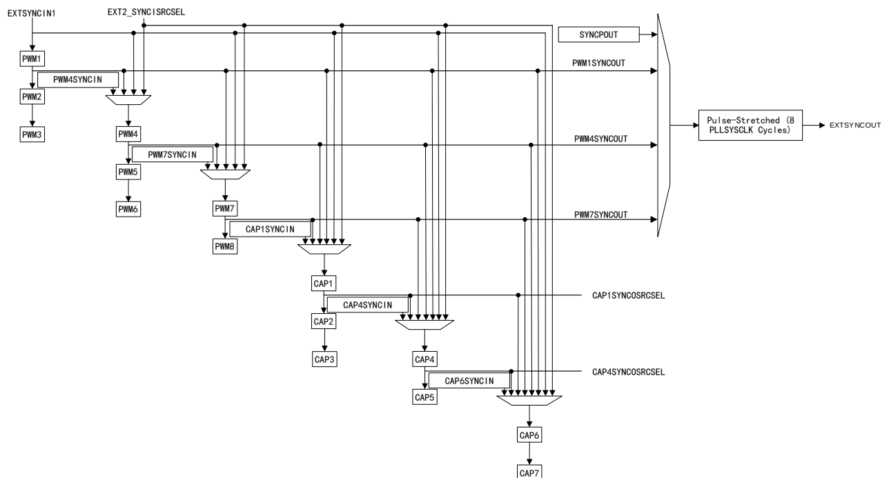
Figure 153 Time Base Counter Synchronization Scheme
