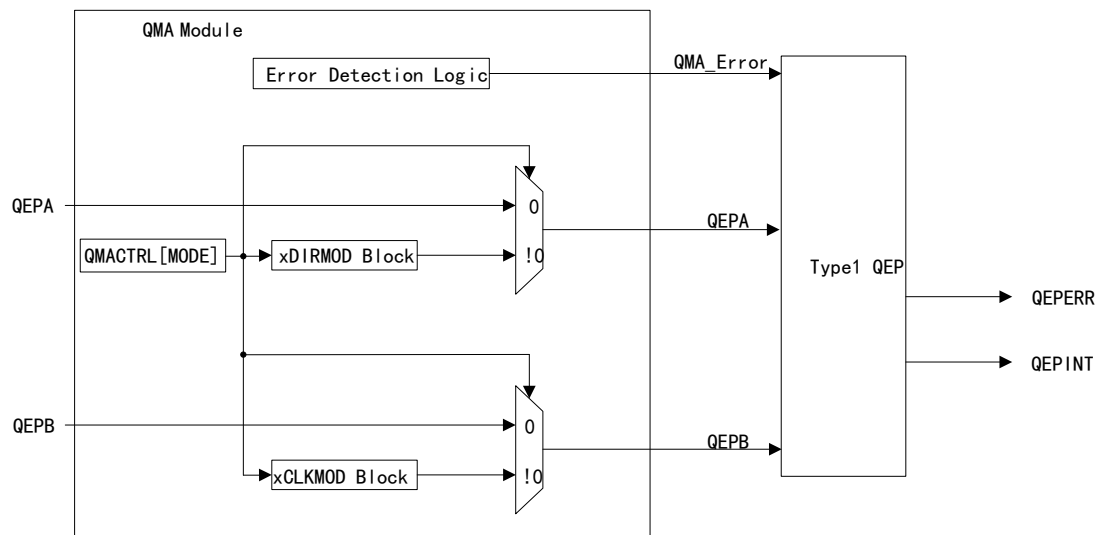
Figure 173 QMA Structure Block Diagram
