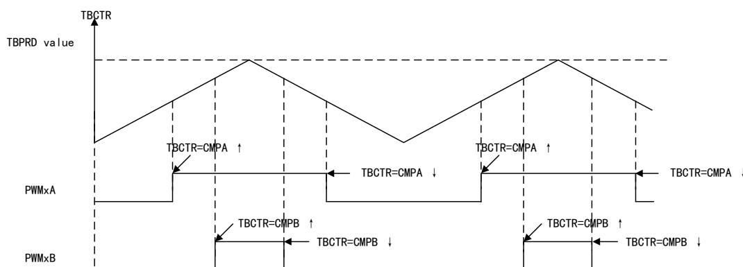
Figure 97 Double-edge Symmetric Waveform Diagram with Independent Modulation on PWMxA and PWMxB in Center-aligned Mode (Low Level is Active)
