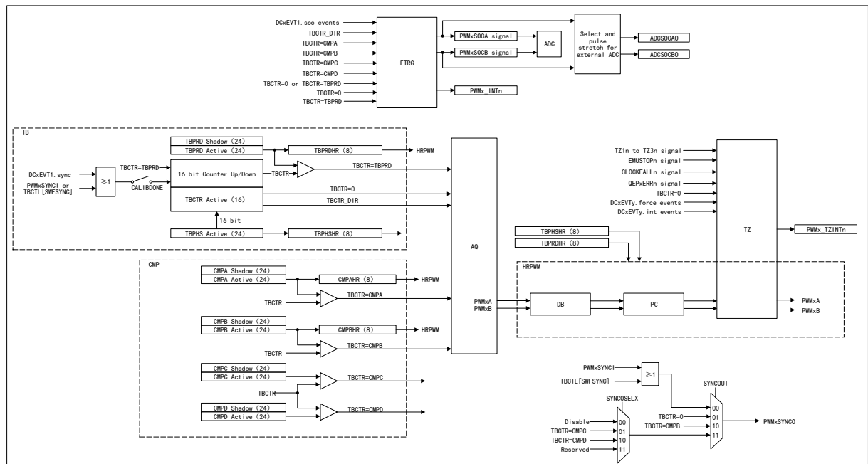
Figure 75 Structure Block Diagram for Interconnection between PWM Module and Key Internal Signals
