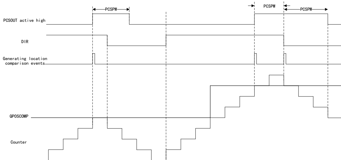
Figure 183 Position Compare Synchronization Output Pulse Extender
