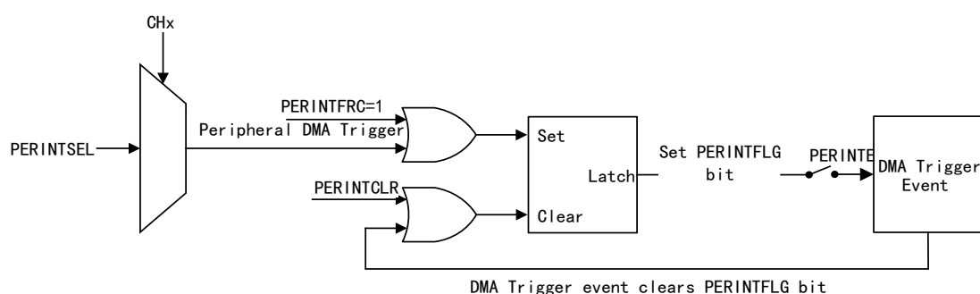
Figure 28 DMA Peripheral Interrupt Triggers Input
