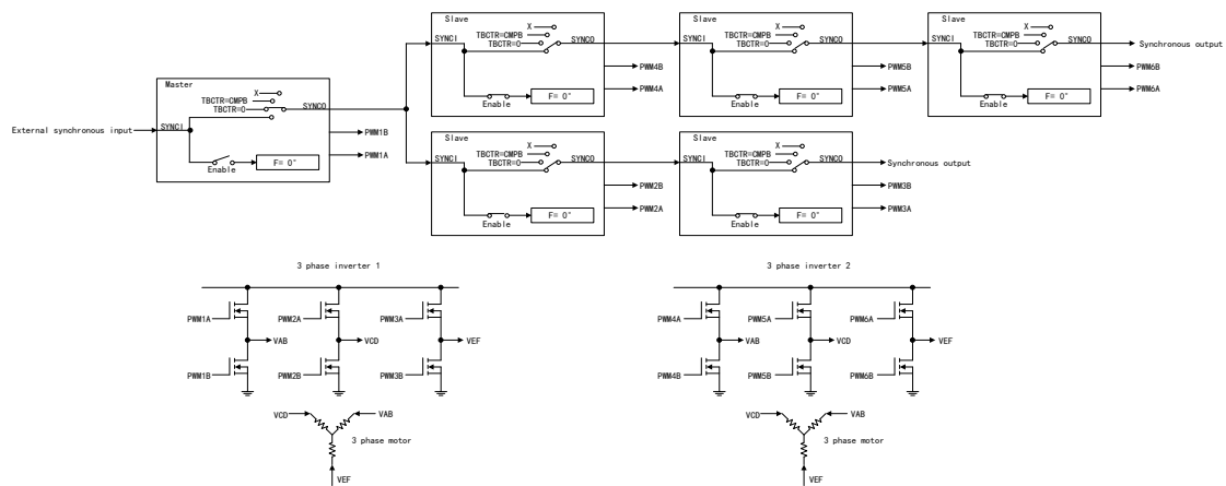
Figure 130 Structure Block Diagram of Dual Three-phase Inverter Stages
