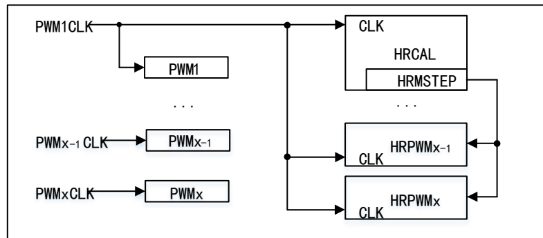
Figure 144 HRPWM and HRCAL Clock Source
