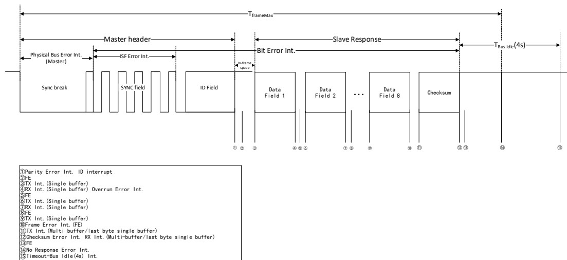
Figure 275 LIN Message Frame Illustrating the Timing and Sequence of LIN Interrupts
