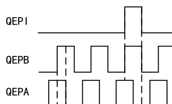
Figure 166 QEPI Waveform Diagram
