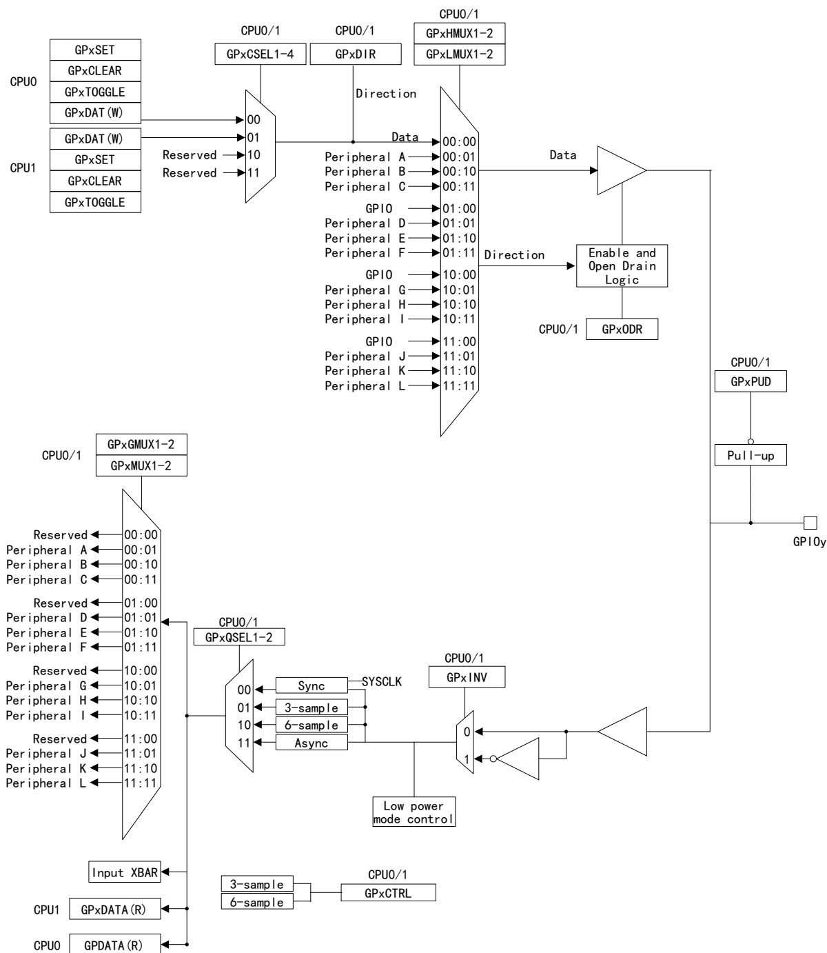
Figure 17 GPIO Structure Block Diagram
