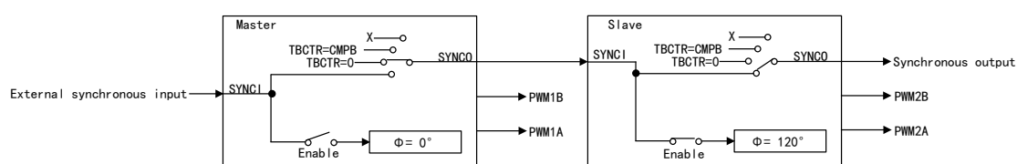
Figure 135 Waveform Diagram for Phase Synchronization between Two PWM Modules
