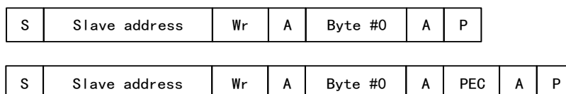
Figure 218 Transmit Byte Message with and without PEC
