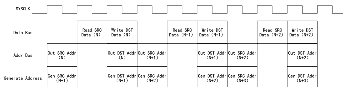
Figure 30 Three-stage Assembly Line DMA Transmission
